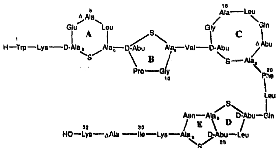
Fig. 1. The schematic chemical structure of subtilin.
